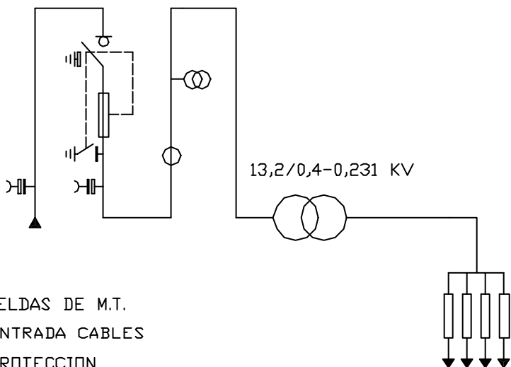
DIAGRAMA UNIFILAR
