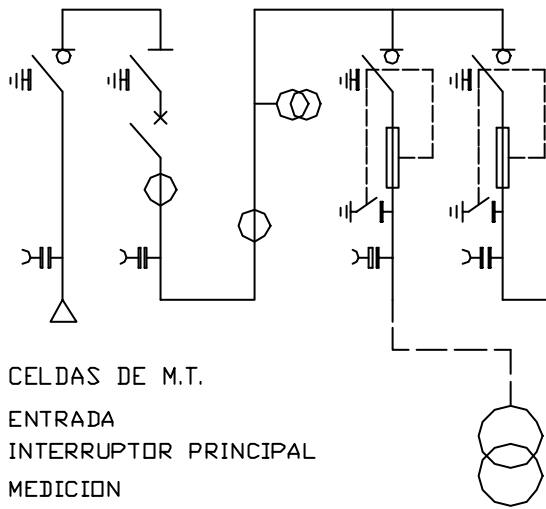
DIAGRAMA UNIFILAR
