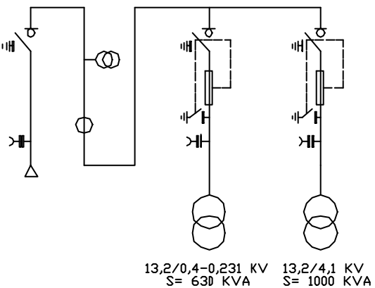
DIAGRAMA UNIFILAR
